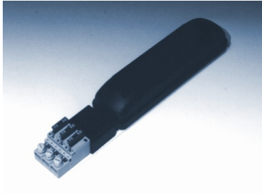
Electronic transformer with secondary fuses (special version for german fairs)
