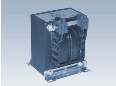
Transformer with terminal blocks
